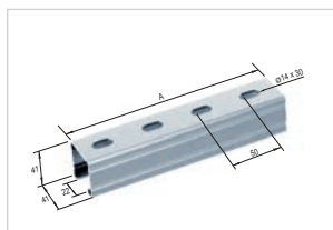
R4141 Rail 41x41
