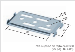
BT Base transversal
