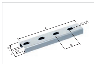
R4121 Rail 41x21
